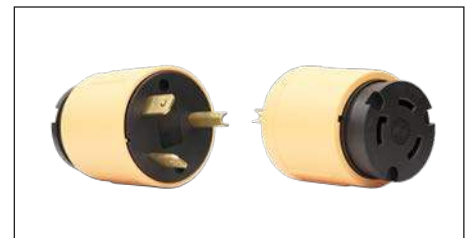
TT-30R to L5-30R Adapter, Front & Back (70137 & 70126 only)
